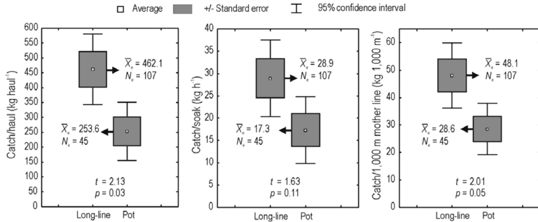
Figure 4. Box plot of yields obtained with long-lines (e) and pots (t).
