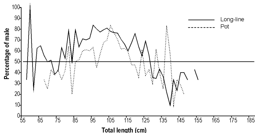
Figure 5. Sexual proportion of the size at catch of Patagonian toothfish obtained with long-lines and pots.
