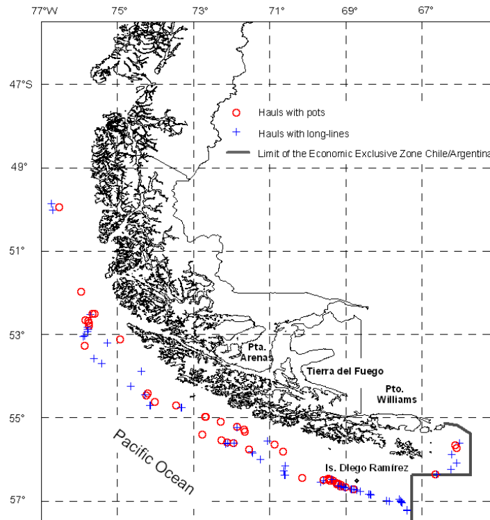
Figure 2. Locations of the fishing hauls done with long-lines and pots during the study period.
