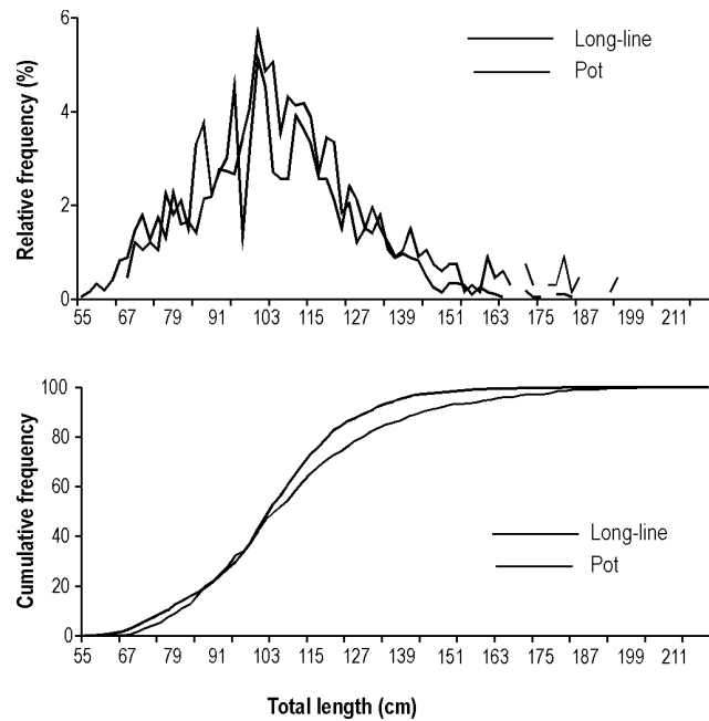
Figure 7. Distribution of relative and accumulated size frequencies in Patagonian toothfish caught with long-lines and pots.
