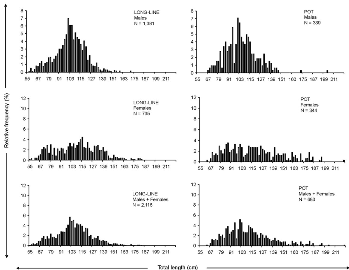
Figure 6. Distribution of size frequencies in Patagonian toothfish by sex and fishing gear.
