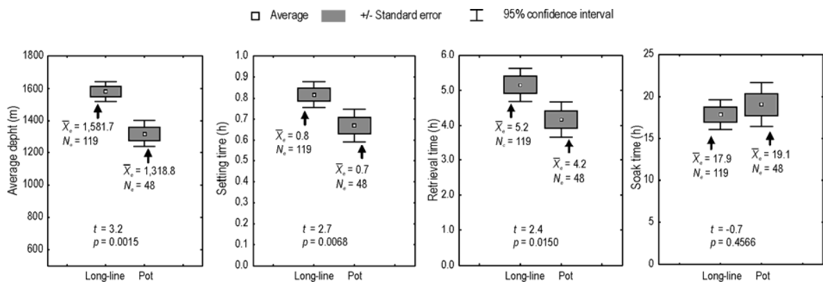
Figure 3. Box plot of operational variables recorded with long-lines (e) and pots (t).
