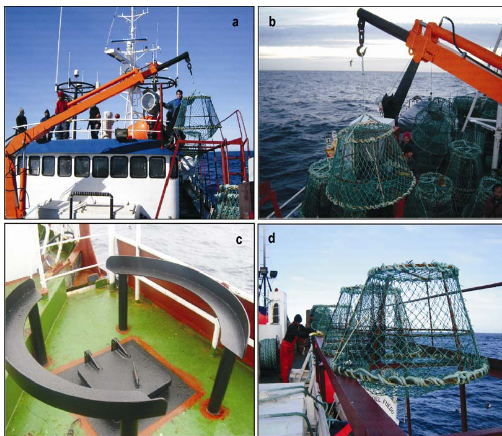
Figure 1. Rigging the vessel to operate with a) pots, b) telescopic crane, c) pot retrieval collar, and d) rail for moving the pots.
